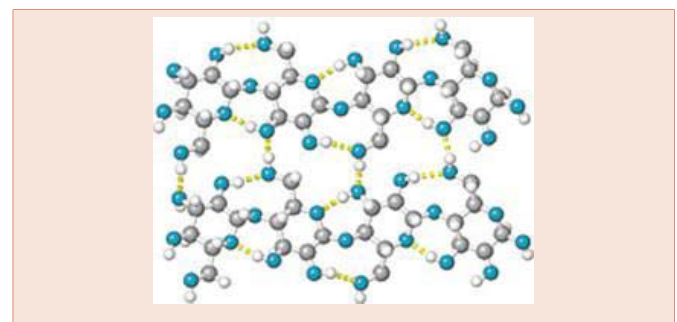
Figure 5: Cellulose fibres.
