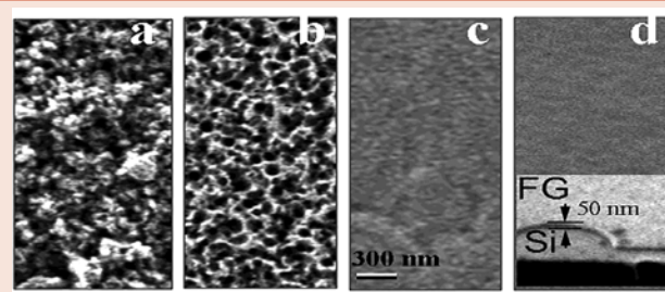
Figure 5: SEM images of the surface of films fluorinated in the aqueous solution of HF during different times. The scales in the images are identical. a – pristine (non-fluorinated) film; b, c, and d – films fluorinated respectively during 2, 10, and 40 days. The inset in Fig. 5 d shows an image of an edge of the film taken at the angle 45° to the surface; the film thickness indicated in the figure was evaluated with allowance for measurement geometry Reprinted with permission from Ref. 56.
