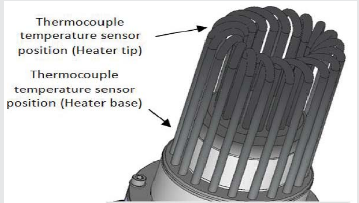
Figure 20: Placement of temperature sensors on the base and tip of the motor heater [19].
