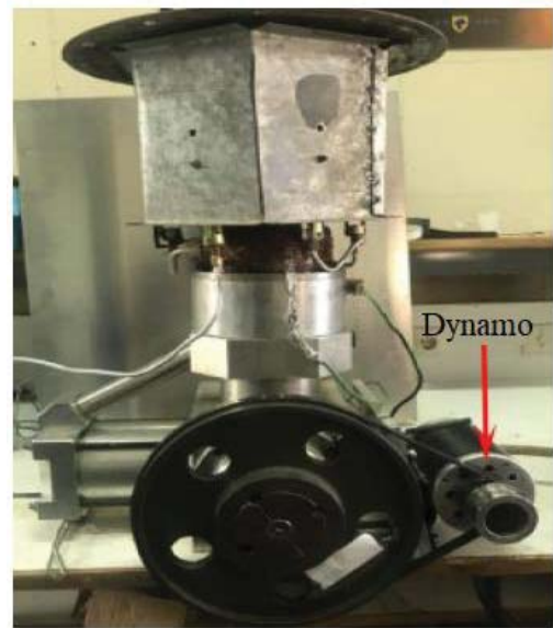
Figure 18: Alternator in Stirling engine and heat chamber.
