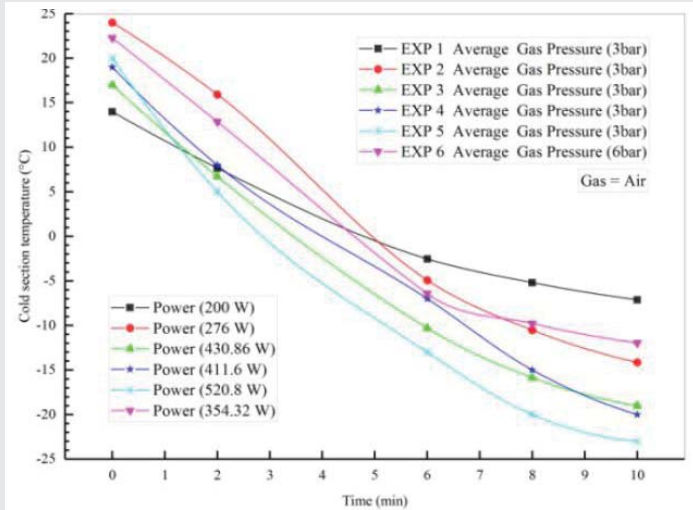
Figure 14: Temperature-time diagram for air gas experiments at different pressures for the Stirling engine in cooling mode [30].
