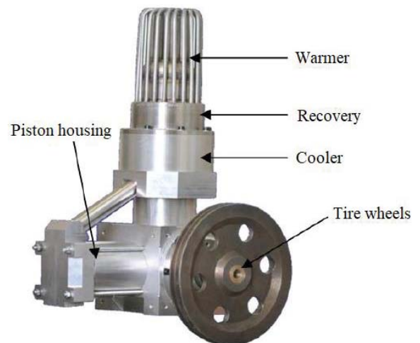
Figure 6: Exterior view of Stirling engine ST-500.
