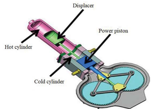
Figure 2: Schematic of beta-type Stirling engine.
