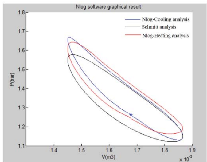
Figure 26: P-V diagram.
