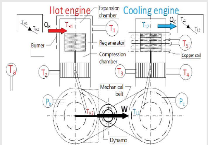
Figure 21: Schematic of Stirling engine coupling ST500 (heat and cooling) to generate cooling.
