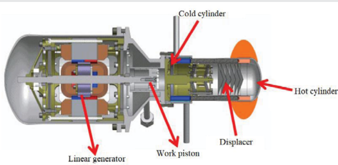
Figure 4: Schematic of free-piston type Stirling engine.
