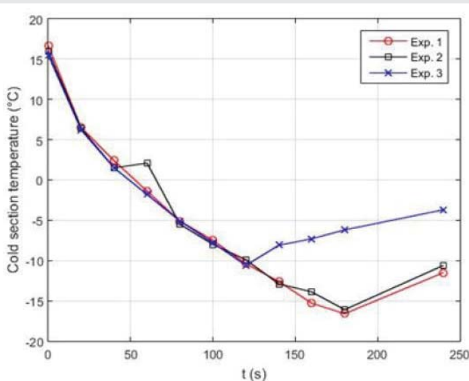
Figure 15: Temperature-time diagram for helium gas experiments [29].
