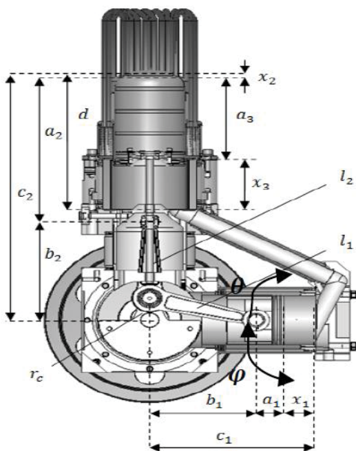
Figure 5: Engine kinematic parameters ST500.
