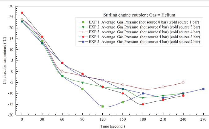
Figure 25: The temp-time diagram for the 5 carried-out tests with Helium gas in varying pressures and the couple state of Stirling engine to produce cooling.
