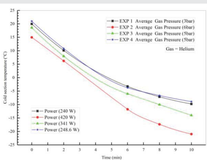
Figure 16: Temperature-time diagram for helium gas experiments at different pressures and cooling engine mode [30].
