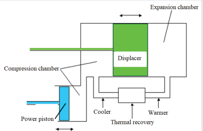
Figure 3: Schematic of gamma type Stirling engine.
