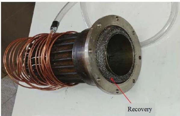
Figure 7: Stirling engine heater with recovery.
