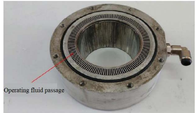
Figure 8: Stirling engine coolant and fluid passage ducts.
