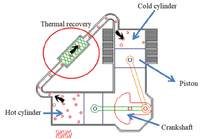
Figure 1: Schematic of Alpha type Stirling engine.
