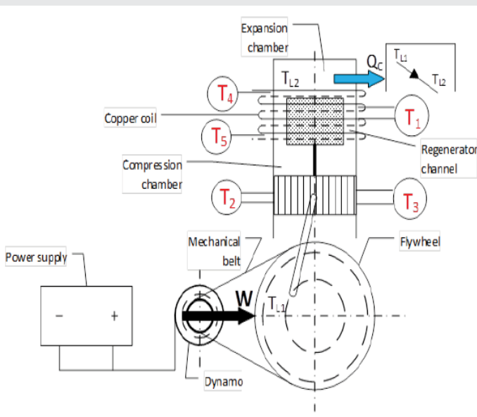
Figure 9: Gamma-type Stirling engine ST500 schema.
