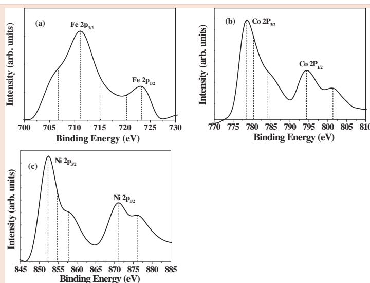
Figure 2: The ex situ (a)Fe, (b) Co, (c) Ni 2p XPS spectra for the as-deposited LiF-MO thin films.
