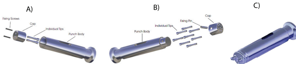
Figure 2: Types of staples used in mini tablet production (6).
