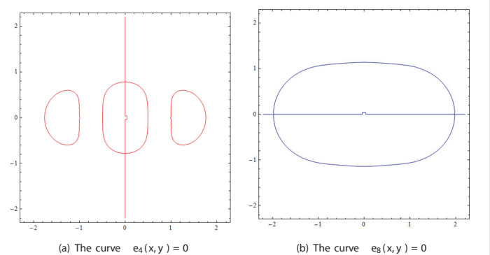
Figure 2: The curves e_4(x, y) = 0 and e_8(x, y) = 0 in the rectangle (x, y) \in [-2.2, 2.2] \times [-2.2, 2.2] .
