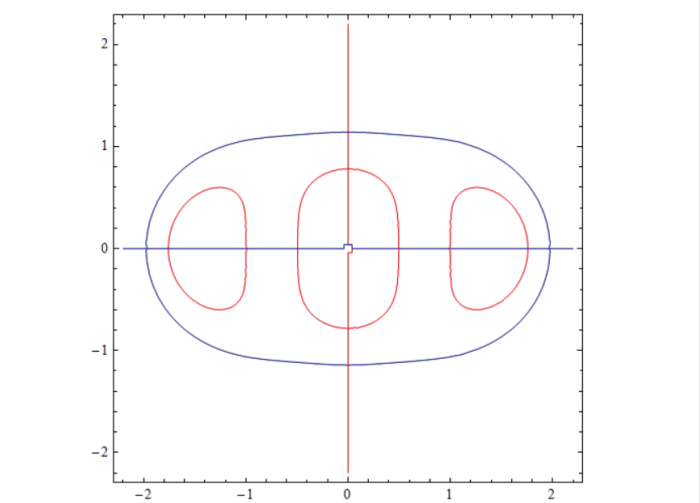
Figure 3: In this picture we can see the six intersection points between the two curves e_4(x, y) = 0 and e_8(x, y) = 0 different from the positions of the primaries, which provide the six central configurations of the circular restricted 4-body problem with three primaries of equal masses at the collinear configuration of the 3body problem and an infinitesimal mass.
